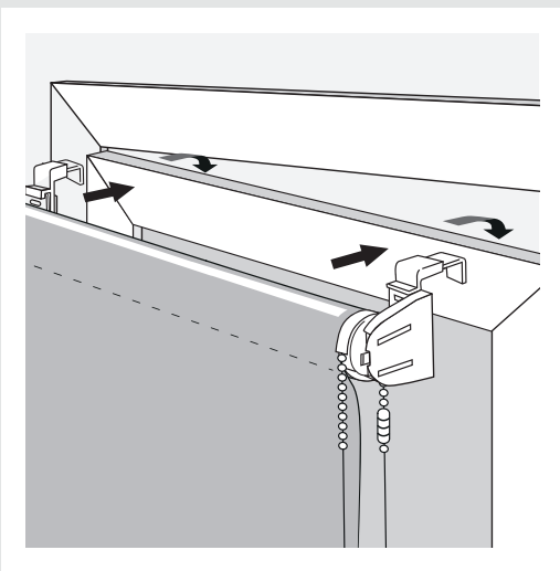
Clip to window frame
